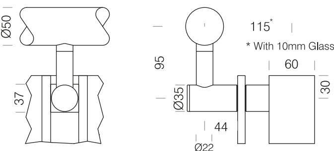
4H Offset Stem Toprail / Single Infill Panel
