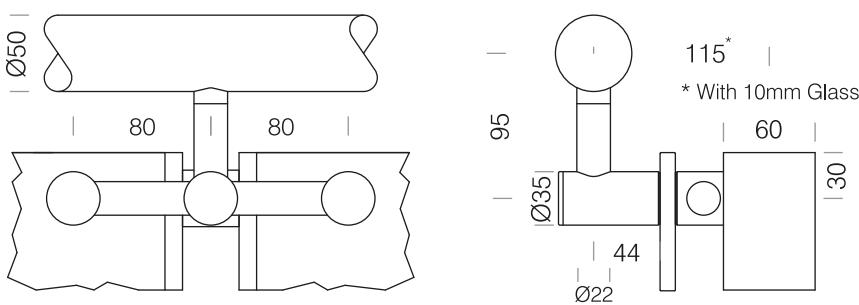
4L Offset Stem Toprail / Double Infill Panel
