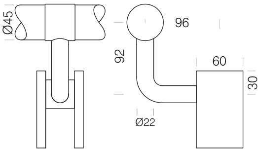
4K Offset Bend Toprail
