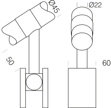
4F Angled Inline Stem Toprail
