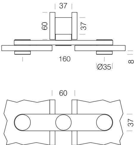
5I Double Offset Fin Panel Holder*
