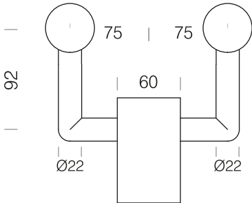
4W Offset Ball Bend Divider Rail
