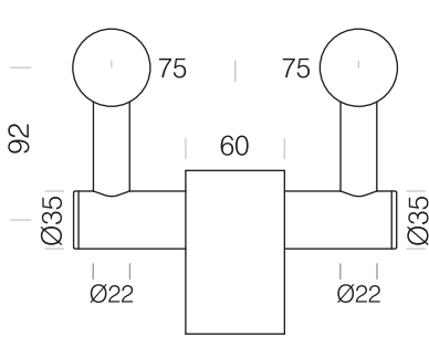
4I Stem Divider Rail
