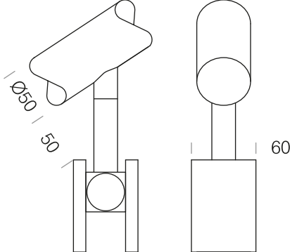
4F Angled Inline Stem Toprail
