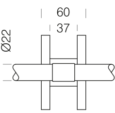
5J Offset Node Midrails
