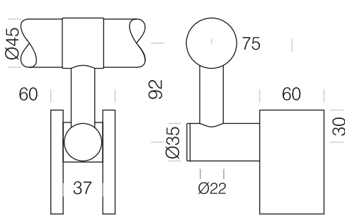
4G Offset Stem Toprail
