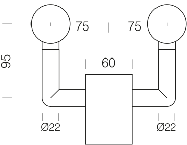
4W Offset Ball Bend Divider Rail
