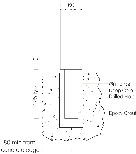
6A Spigot Fixing
