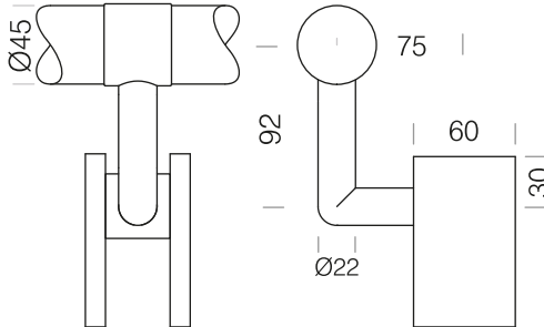
4V Offset Ball Bend Toprail
